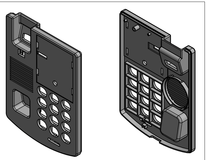
3D View (1 : 2)
