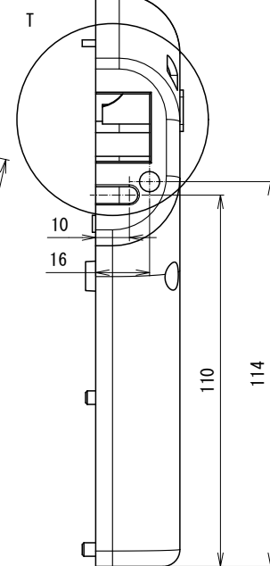
K (1:1)
