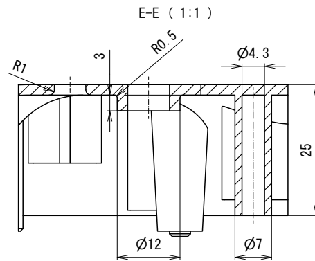
E-E (1:1)
