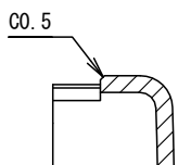
M-M (1:1)
