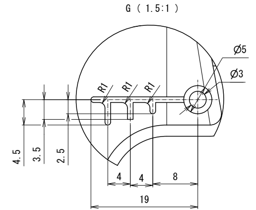
G (1.5:1)
